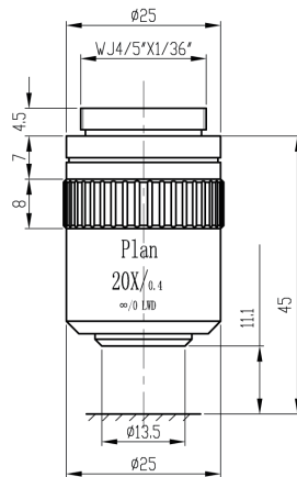
METALLURGICAL BRIGHT FIELD 20X
