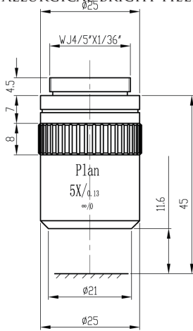
METALLURGICAL BRIGHT FIELD 5X
