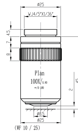
METALLURGICAL BRIGHT FIELD 100X
