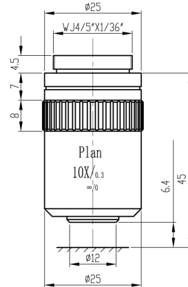
METALLURGICAL BRIGHT FIELD 10X
