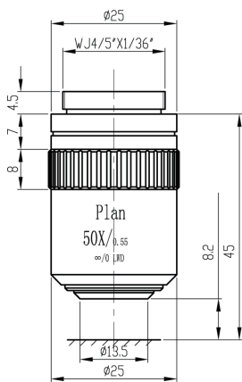
METALLURGICAL BRIGHT FIELD 50X
